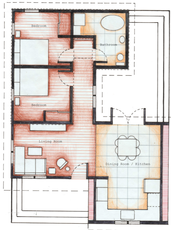
Ground Floorplan - 1/4"=1'
