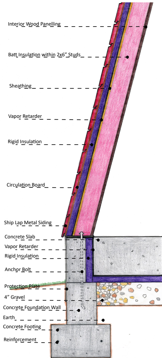
A-Frame Wall Section Detail - 3"=1'
